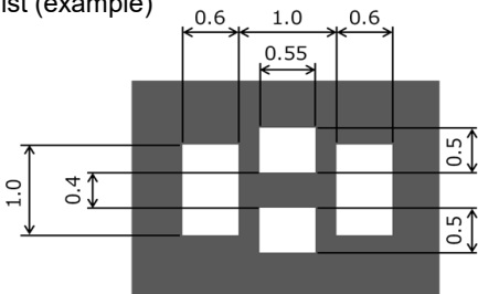
Solder resist (example)
