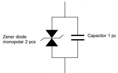
[Equivalent Circuit]
