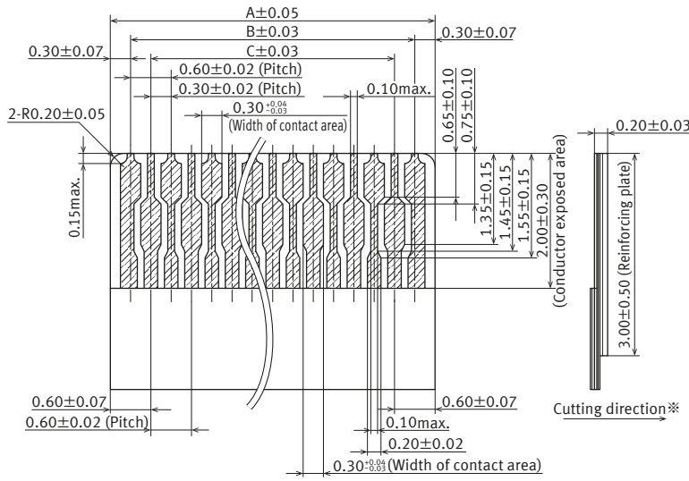
Dimension table
