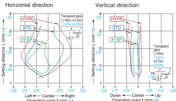
FD-L31A Reflective type
