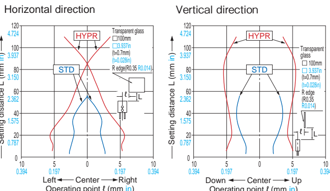
FD-L32H Reflective type
