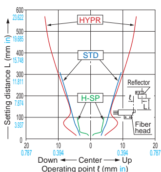
Retroreflective type
