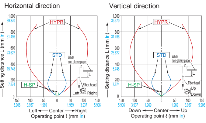
FD-S33GW Reflective type FD-S60Y Reflective type
