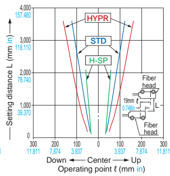
Thru-beam type
