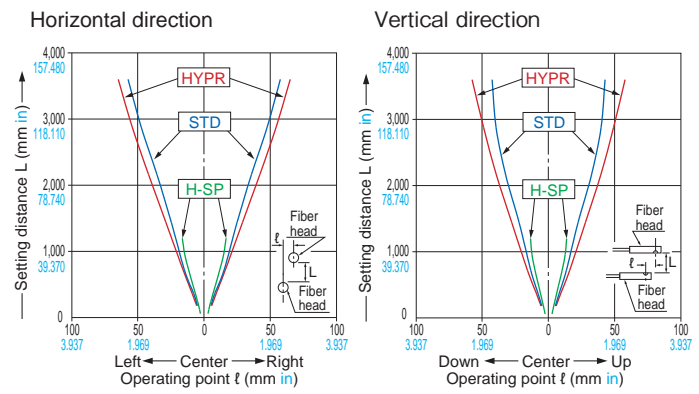
FT-L80Y Thru-beam type
