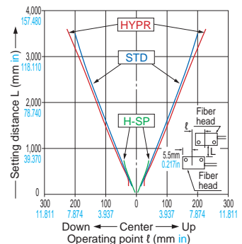
FT-Z30E Thru-beam type
