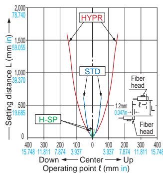
FT-Z30E Thru-beam type
