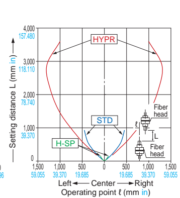
FT-R42W Thru-beam type
