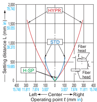
FT-Z30 Thru-beam type
