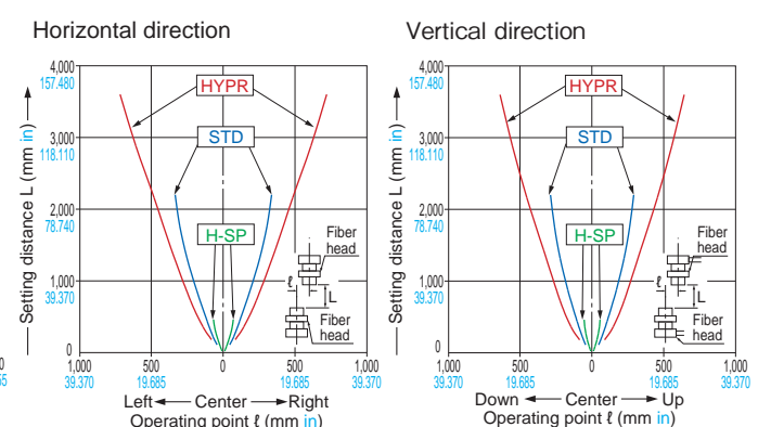
FT-R42W Thru-beam type
