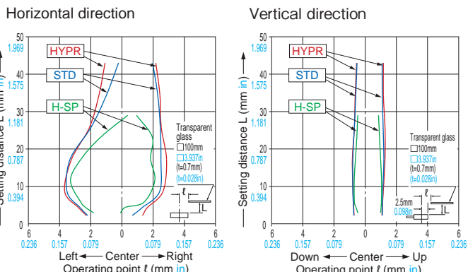
FD-L30A Reflective type
