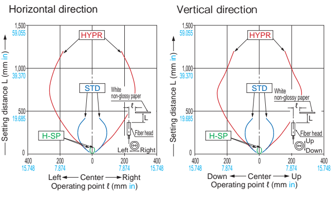
FD-S33GW Reflective type FD-S60Y Reflective type
