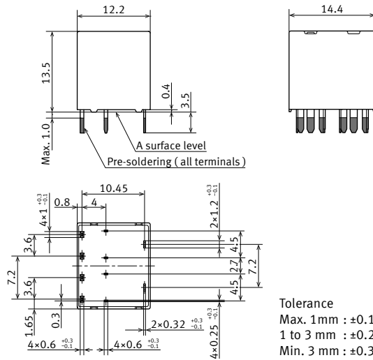
External dimensions
