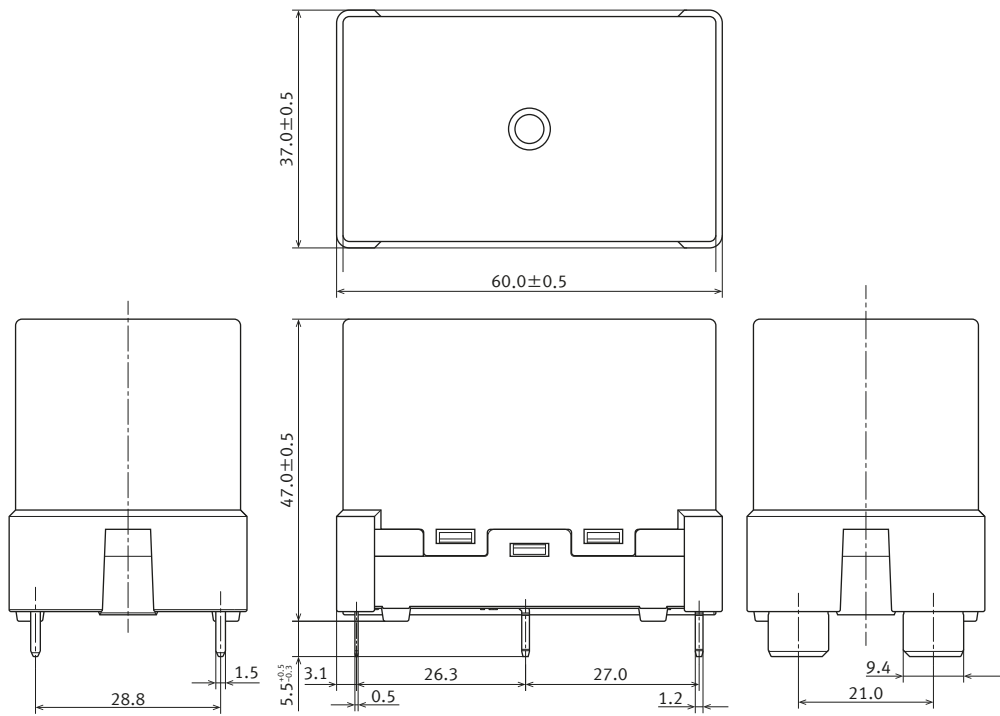
External dimensions
