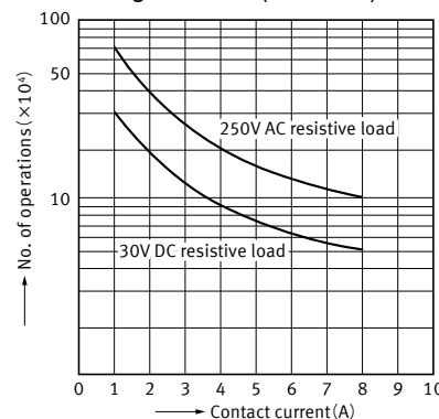
2-2. Switching life curve (1 Form A, 1 Form B) 2-3. Switching life curve (2 Form A)
