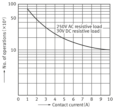
2-1. Switching life curve ( 1 Form A )
