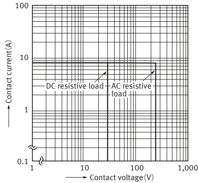
1-1. Max. switching capacity ( 1 Form A ) 1-2. Max. switching capacity ( 1 Form A 1 Form B, 2 Form A )
