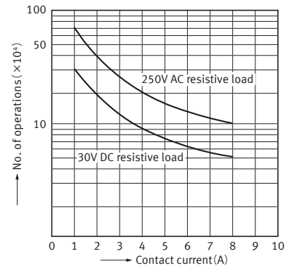
2-3. Switching life curve ( 2 Form A )
