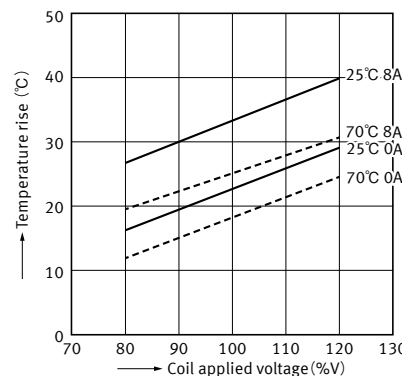
3-3. Coil temperature characteristics (2 Form A: Average)
