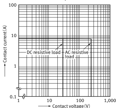
1-2. Max. switching capacity (1 Form A, 1 Form B, 2 Form A)
