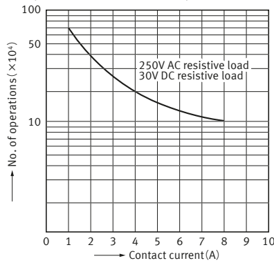
2-2. Switching life curve ( 1 Form A 1 Form B )
