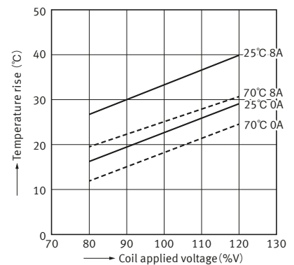
3-3. Coil temperature characteristics ( 2 Form A: Average )
