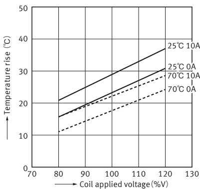
3-1. Coil temperature characteristics ( 1 Form A: Average )
