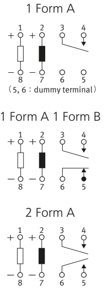
Schematic ( BOTTOM VIEW ) ( Reset )
