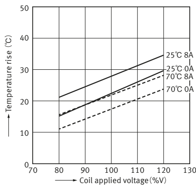
3-2. Coil temperature characteristics ( 1 Form A 1 Form B: Average )
