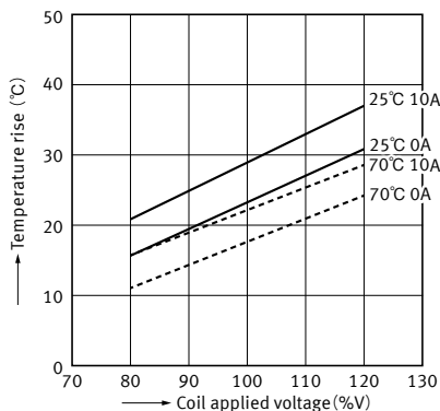
3-1. Coil temperature characteristics (1 Form A: Average)
