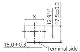
Diagram of recommended for panel mounting holes
