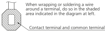
Soldering position
