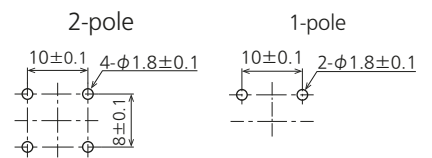
P/C board pattern
