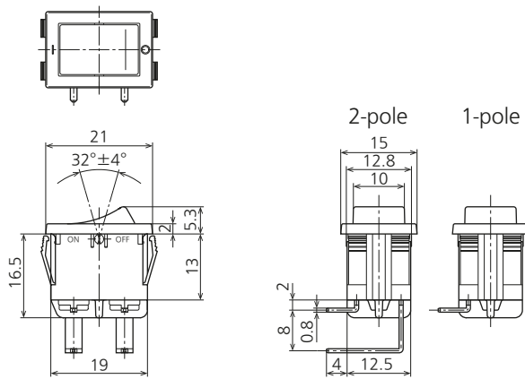
External dimensions
