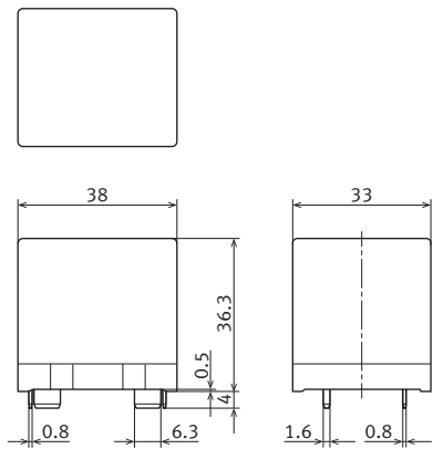
External dimensions
