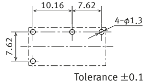
Recommended PC board pattern ( BOTTOM VIEW )
