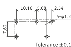
Recommended PC board pattern ( BOTTOM VIEW )
