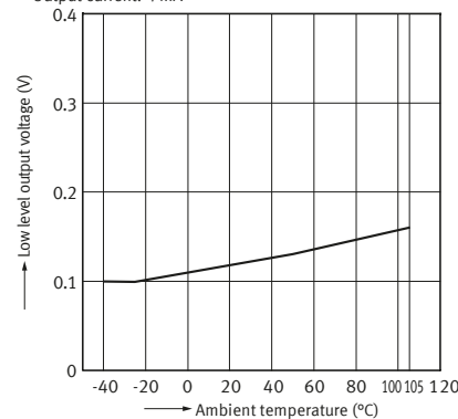
5. Low level output voltage vs. ambient temperature characteristics
