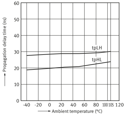
7. Propagation delay time ( H → L/L → H ) vs. ambient temperature characteristics
