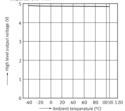
6. High level output voltage vs. ambient temperature characteristics
