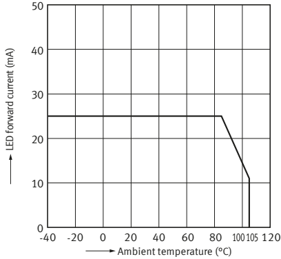
1. LED forward current vs. ambient temperature characteristics
