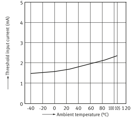
3. Threshold input current vs. ambient temperature characteristics
