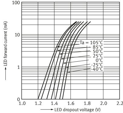
2. LED forward current vs. LED drop out voltage characteristics
