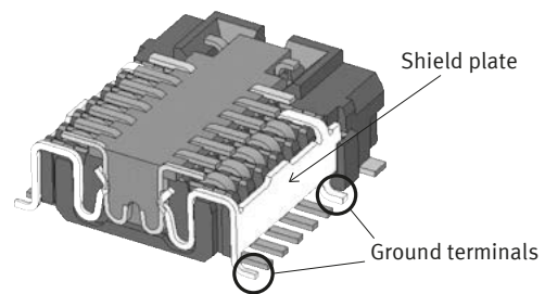
〈Ground terminal cross-section diagram〉
