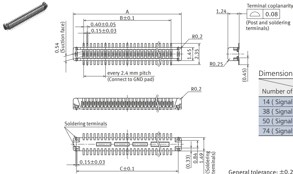
External dimensions
