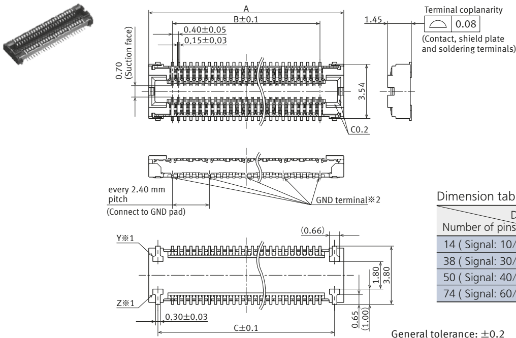
External dimensions
