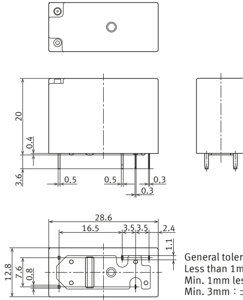
External dimensions
