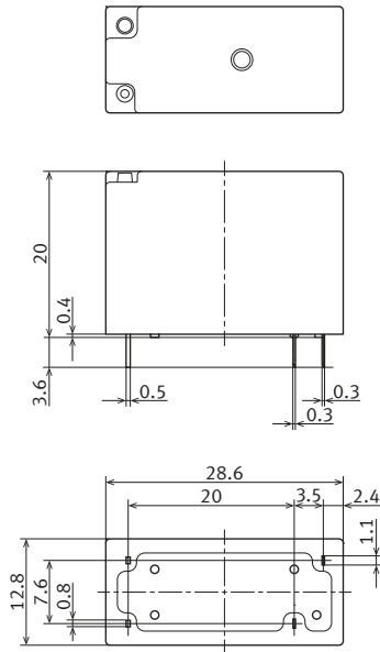
External dimensions
