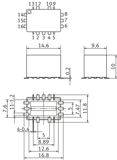
External dimensions
