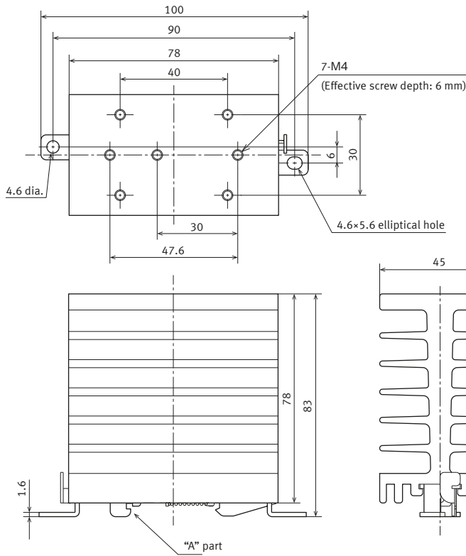
External dimensions
