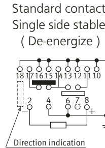
1 coil latching ( Reset )
