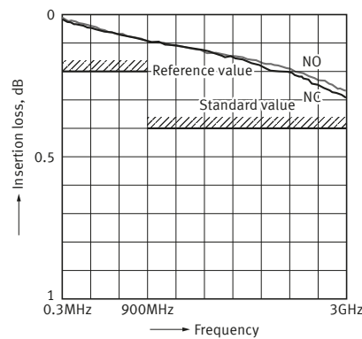
Insertion loss characteristics (without D.U.T. board' s loss)
