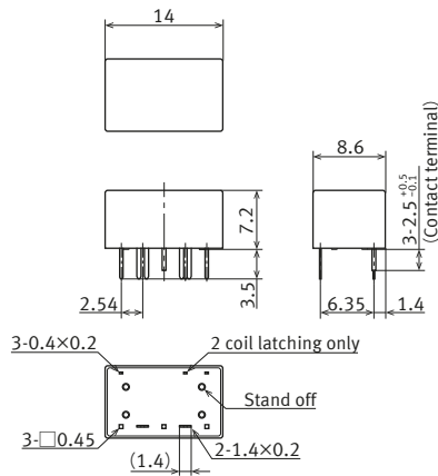
External dimensions
