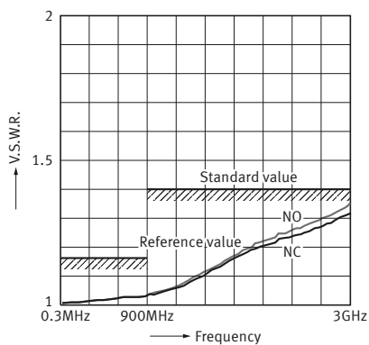
V.S.W.R. characteristics
