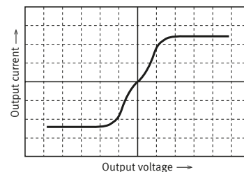
V-I Characteristics
