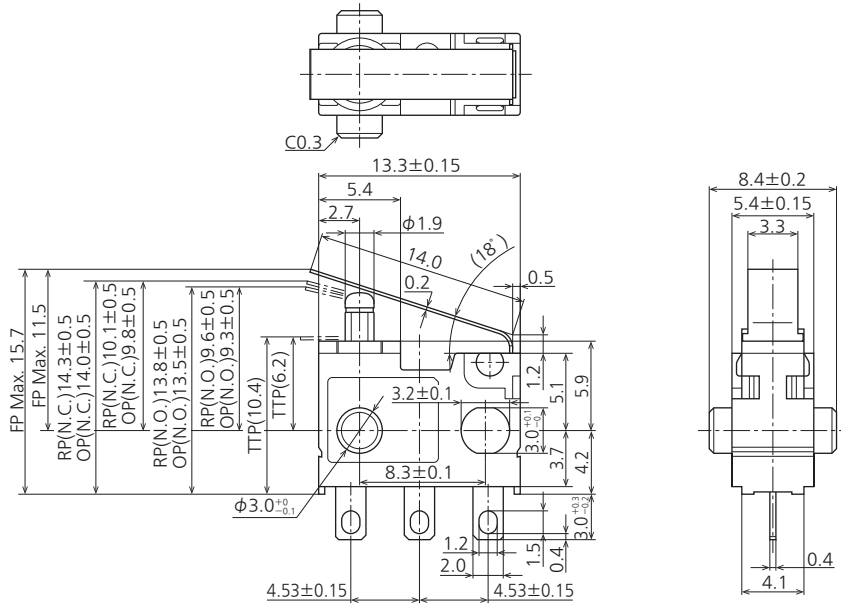
External dimensions
