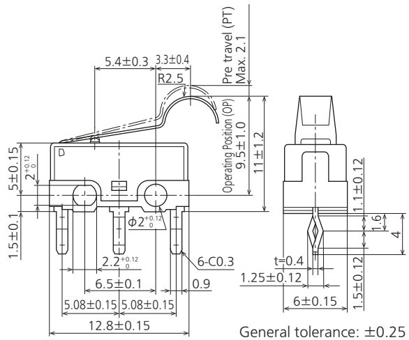
External dimensions
