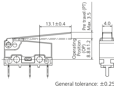
External dimensions
