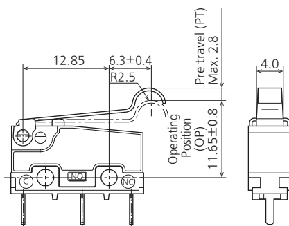
External dimensions
