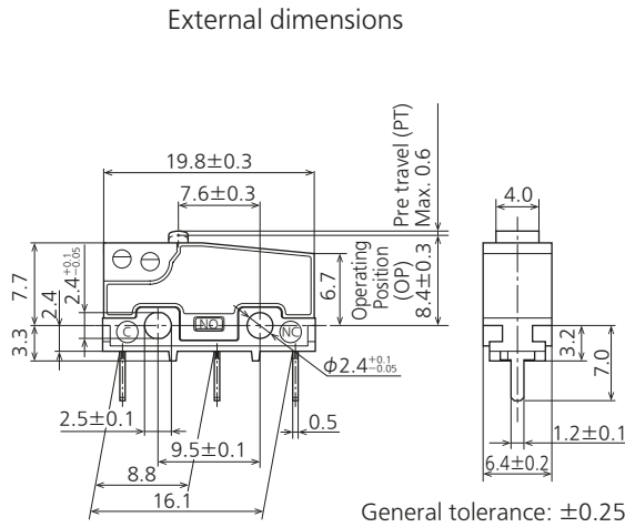
External dimensions
