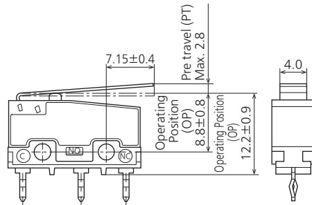
External dimensions
