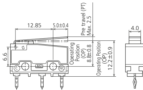
External dimensions
