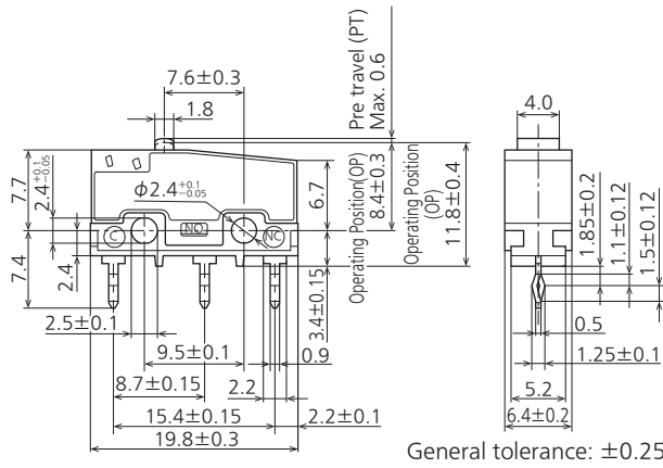
External dimensions
