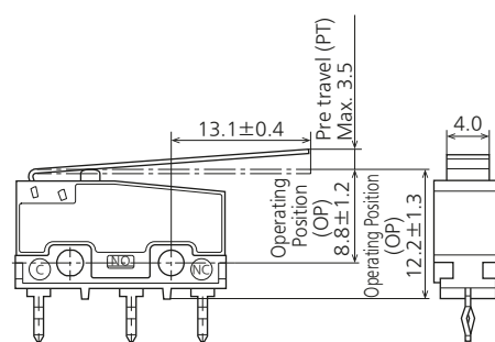
External dimensions
