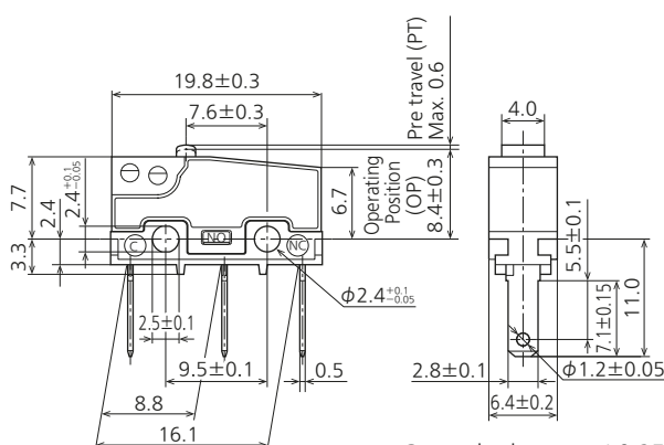
External dimensions
