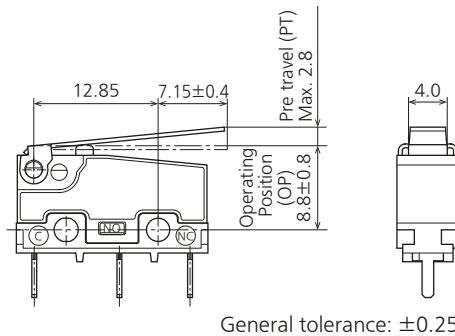
External dimensions
