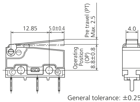
External dimensions
